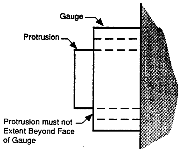
Figure 2 Protrusion Test
