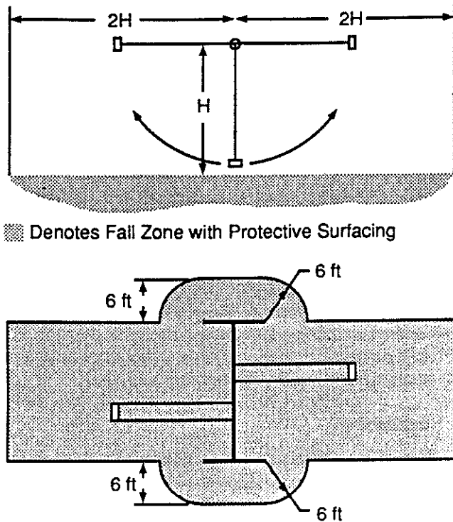
Figure 17 Fall Zone for Single Axis Swings
