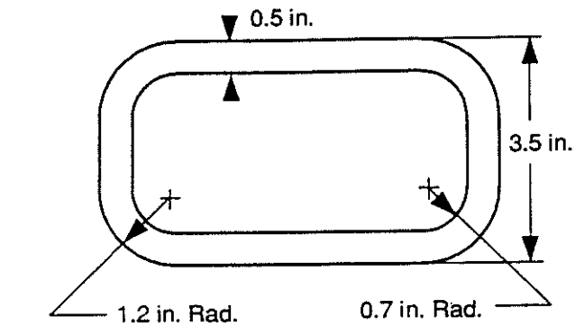
Figure B-7 Small Torso Probe
