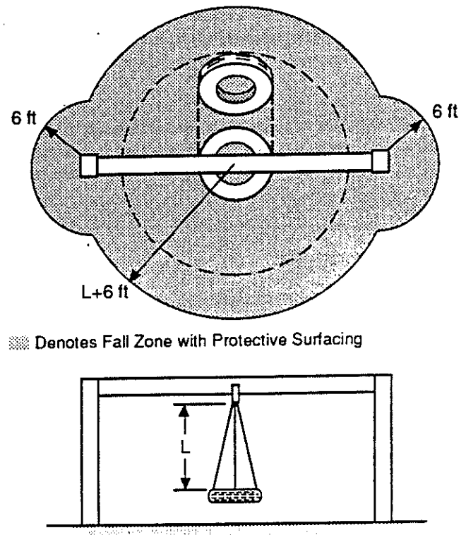
Figure 18 Fall Zone for Multi Axis Tire Swings
